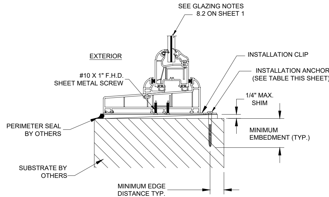
A 5 ANCHOR DETAIL INSTALLATION CLIP FRAME SILL
