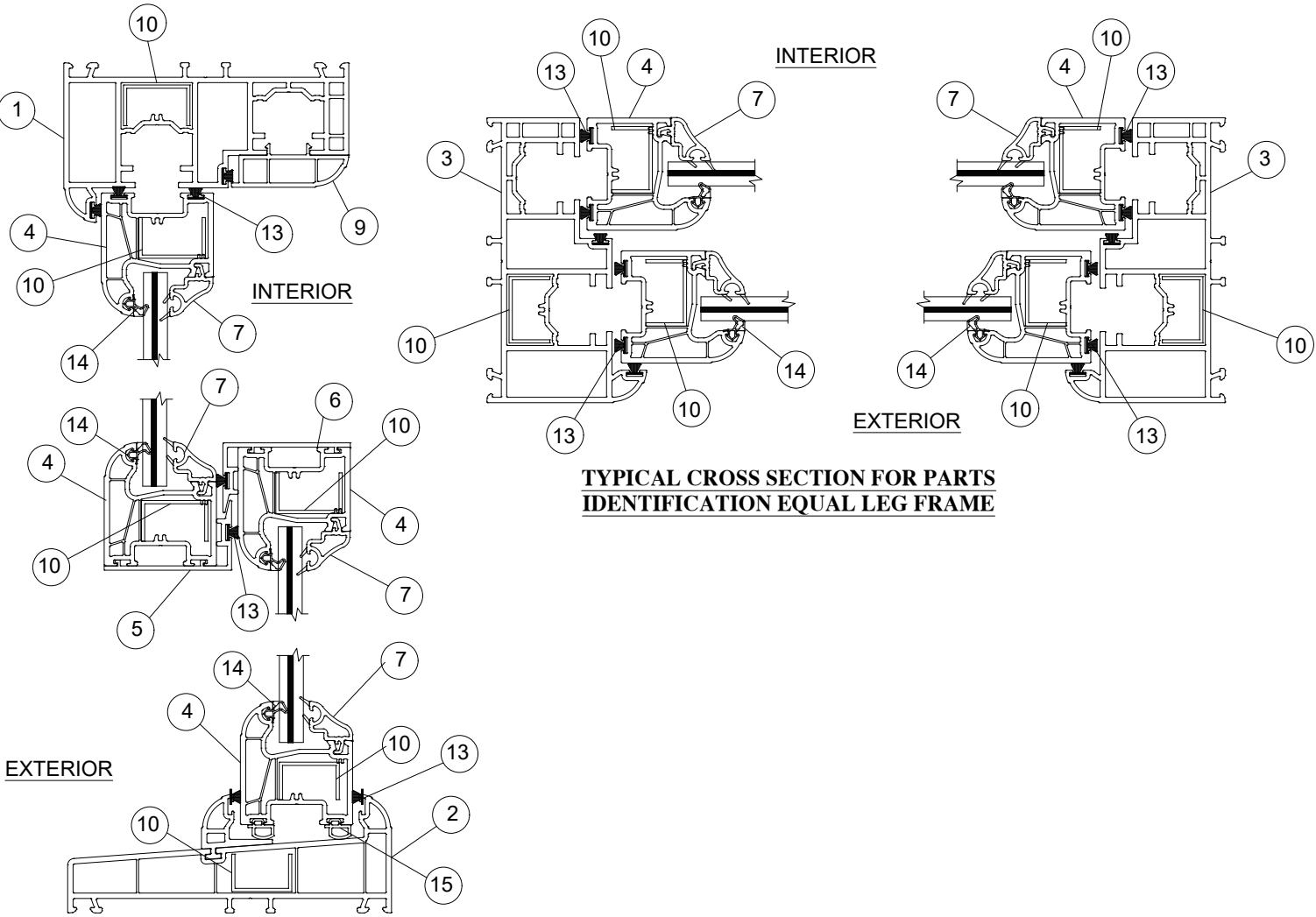
TYPICAL CROSS SECTION FOR PARTS IDENTIFICATION EQUAL LEG FRAME
