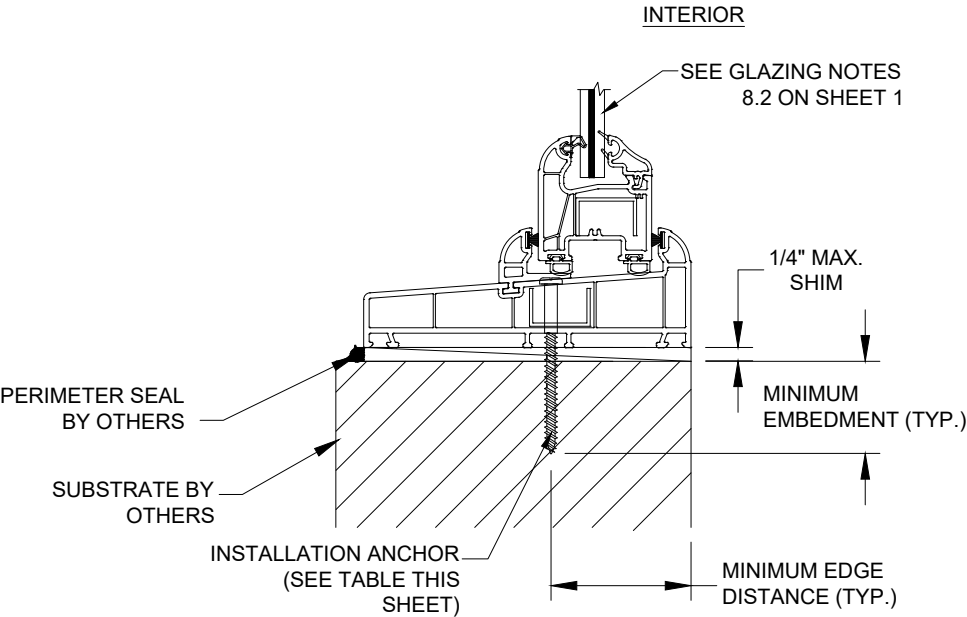
A 6 ANCHOR DETAIL THROUGH FRAME FRAME SILL
