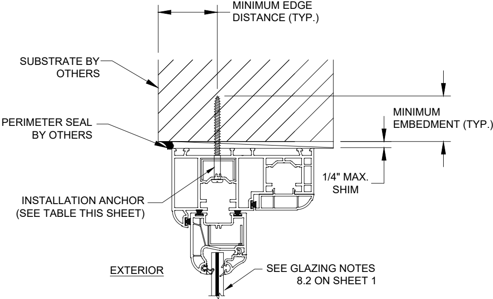
B 6 ANCHOR DETAIL THROUGH FRAME FRAME HEAD
