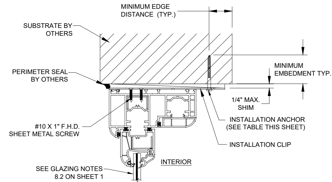
B 5 ANCHOR DETAIL INSTALLATION CLIP FRAME HEAD
